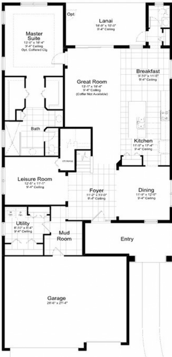
1ST FLOOR
