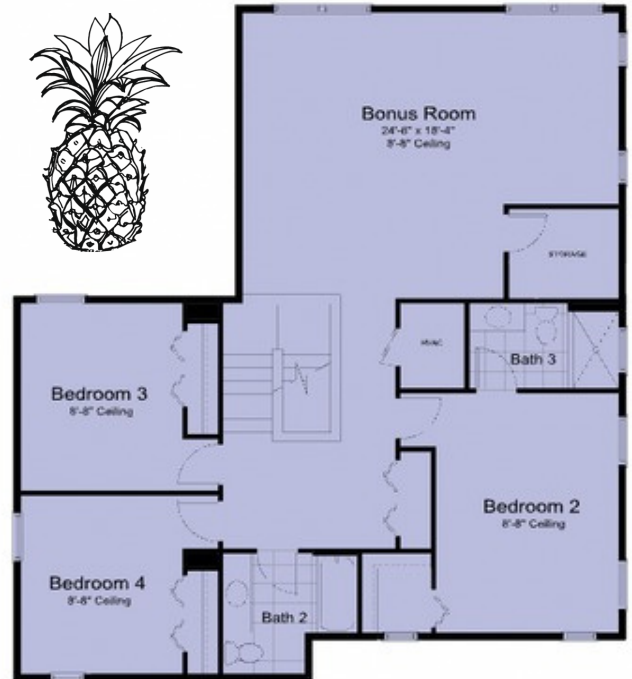
2ND FLOOR
